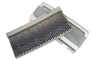
Jet Engine Turbine shroud
